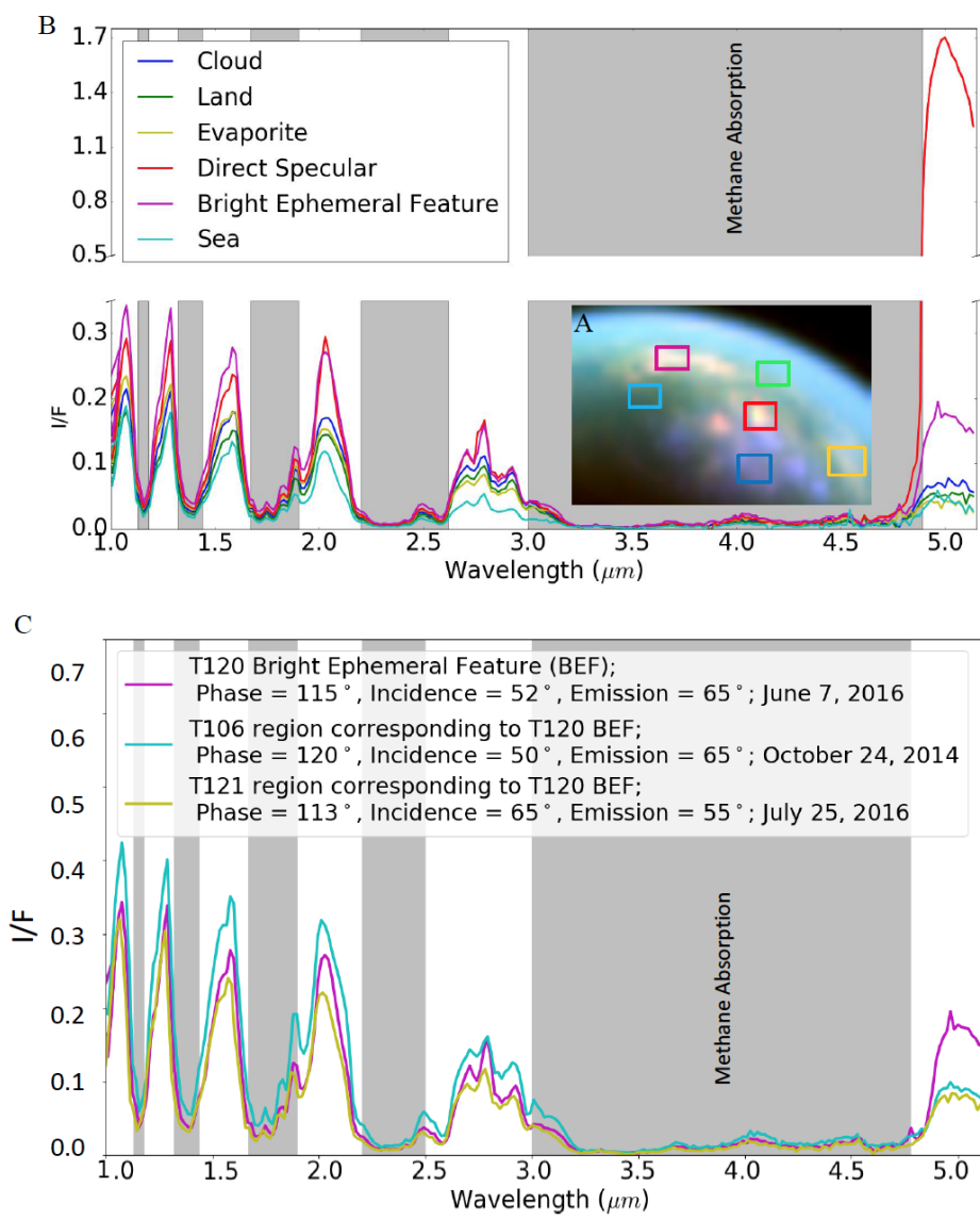
Figure 3. A) The colored boxes correspond to the different regions in the T120 observations: dark blue (clouds), green (land), light blue (sea), red (specular reflection), magenta (BEF), and yellow (evaporites). B) The spectra corresponding to the regions in similar colors as the boxes in A. Grey solid boxes show spectral regions affected by methane absorption and thus blocked by Titan’s atmosphere. C) Shows the spectra for the location of the BEF. The slightly higher reflectance at shorter wavelengths of the T106 observation (cyan) is because of the higher emission angles. The magenta spectrum corresponds to the BEF during the T120 June 2016 flyby which is distinctly brighter than other spectra at 5 \mu m. The yellow spectrum indicates reflectances for the same region three Titan days later during the T121 July 2016 flyby.
