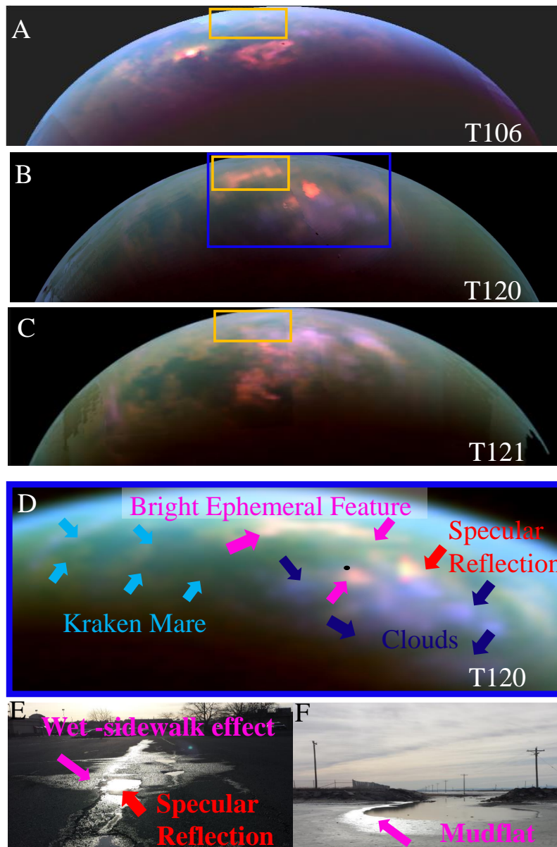
Figure 1. VIMS wet-sidewalk color composite (R:5 \mu m, G: 2.7 \mu m, B:2 \mu m) of Titan's north polar region showing the region corresponding to the BEF in the flybys A) T106, 24 October, 2014 B) T120, 07 June, 2016, and C) T121, 25 July, 2016. The yellow box in 1C shows the disappearance of the Bright Ephemeral Feature (BEF) three Titan days later (See Table 1). D) Zoomed- in view of the north polar region from the T120 flyby annotated to identify the features. The BEF is marked by magenta arrows in the figure. The black dot marks the north pole. E) Analog for the T120 BEF on a cloudy day after rainfall. The specular reflection at the boundary of a puddle can be seen as a bright speck while the road's wetted surface is reflecting broadly at the right geometries. F) Analog for the T120 BEF as mudflat in Utah's Bonneville salt flats
