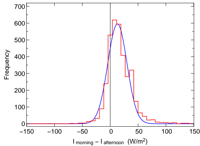
Figure 1. Difference of morning and afternoon irradiance measurements at MLO and airmass 2 for days where both were available (red histogram), showing that morning values are on average larger than afternoon values. The blue curve shows a Gaussian function fit to the data with a peak at 12.9 \text{ W m}^{-2} and a width \sigma = 17.29 \text{ W m}^{-2} .
