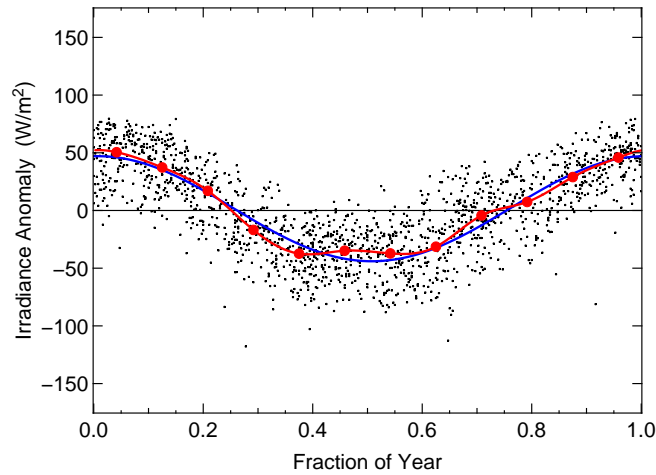
Figure 4. Average seasonal cycle in the terrestrial irradiance at MLO and airmass 2 computed from the irradiance data in the years 2000-09 ( small black squares ) and after removing a linear long-term trend. The filled red circles are the monthly medians while the red line shows a fit of cubic splines with periodic boundary conditions through the monthly medians. The blue line indicates the expected seasonal irradiance variations due to Earth’s orbital motion.
