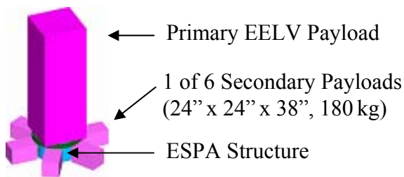
Figure 14. EELV Payloads and ESPA Structure
