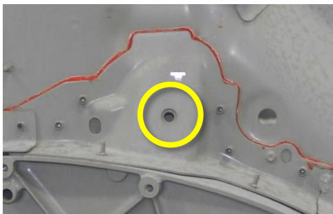
✗ Figure 3 (2nd row lower seat belt hole in 2 nd generation rear node)
