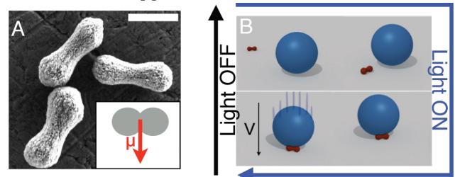
Figure 1. (A) SEM picture of the hematite peanut particles. Scale bar is 1 \mu\text{m} . Inset shows the direction of the permanent magnetic moment \mu of the particle, perpendicular to the long axis. (B) Schematic of docking. Under activation by an external blue light and steering by a magnetic field, a hematite particle docks with a passive sphere and transports it. This scenario is reversible: when the light is turned off, the hematite particles release the cargo and diffuse away.
