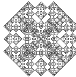
Fig. 20. A perfect 383 \times 383 parity pattern.
