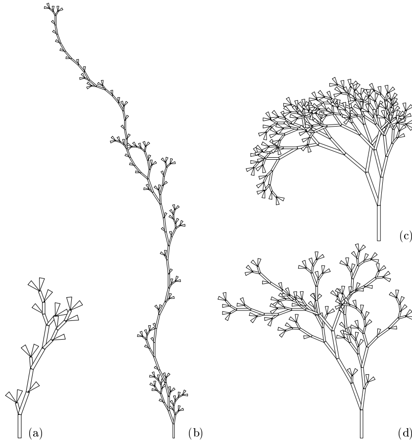
Fig. 42. “Organic” illustrations of binary trees.
