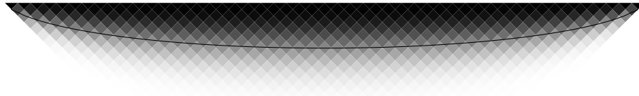
Fig. 36. The shape of a random 50-node forest.
