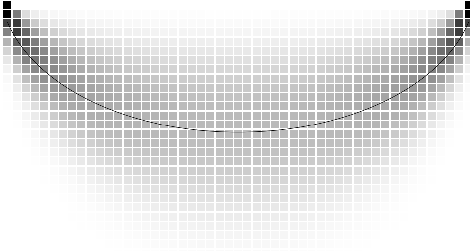
Fig. 38. Locations of the external nodes in a random 50-node binary tree.
