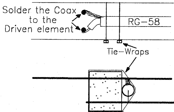
Driven Element Detail
