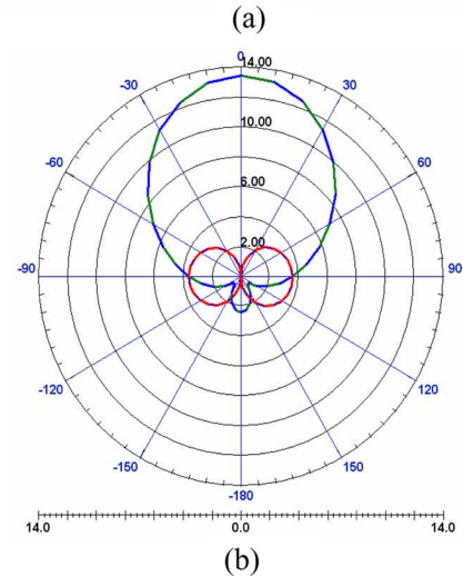
Fig. 6. (a) Complex input impedance values, and (b) far-field E-field (blue) and H-field (red) patterns for Design 6.
