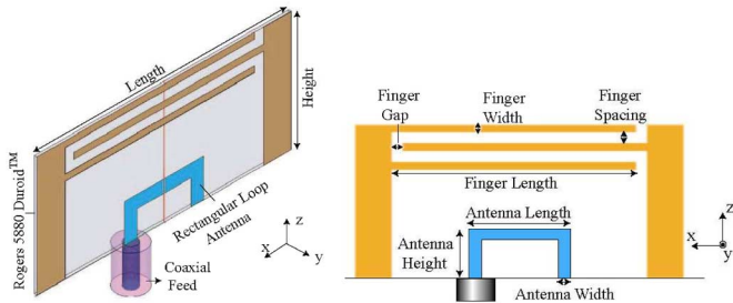
Fig. 5. Geometry and detailed specifications of each design variable for the 2D magnetic-based EZ antenna that incorporates an interdigitated capacitor.
