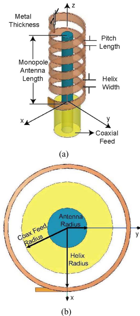
Fig. 8. Geometry and detailed specifications of each design variable for the 3D electric-based EZ antenna (a) 3D view and (b) 2D cross-sectional view.
