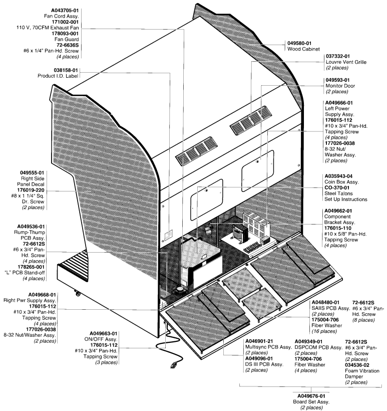
Figure 4-1 Cabinet-Mounted Assemblies, Rear View, Continued A049570-01 D
