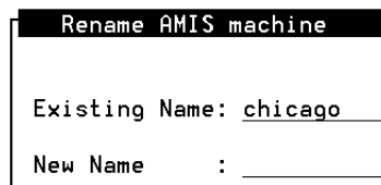
Figure 5-26. Rename AMIS Machine Screen
