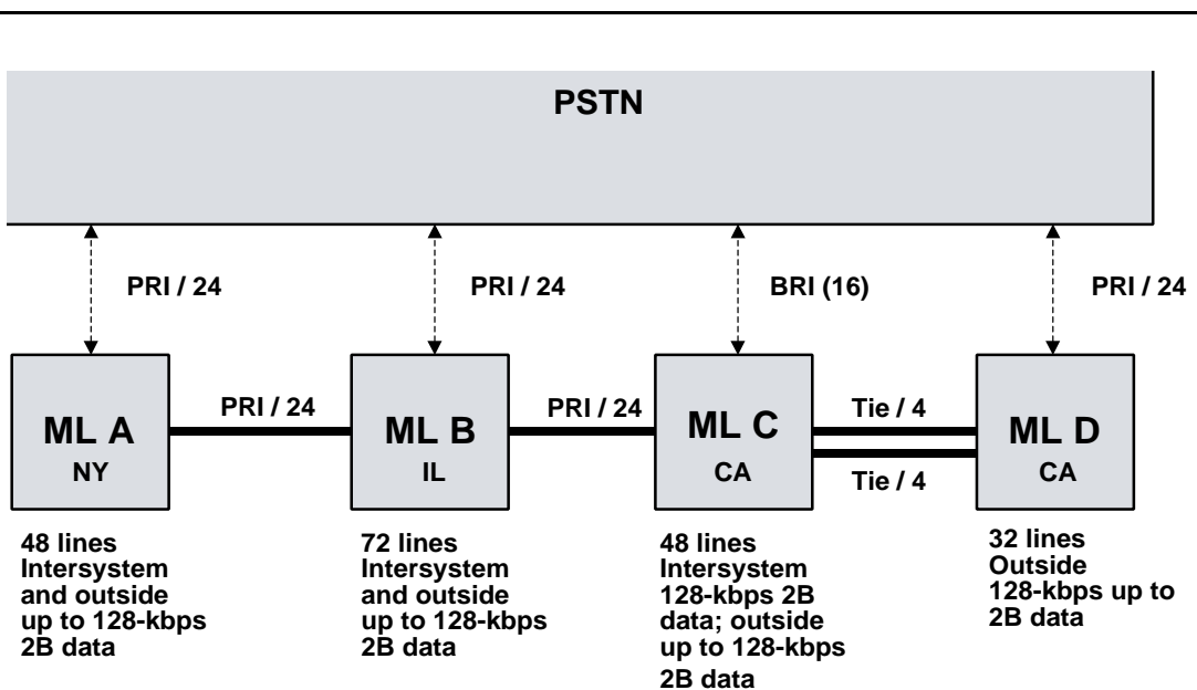
Figure 1-4. Series Configuration: Four Systems
