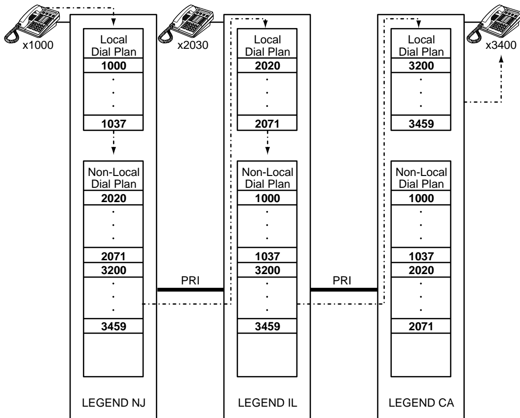
Figure 1-7. Uniform Dial Plans
