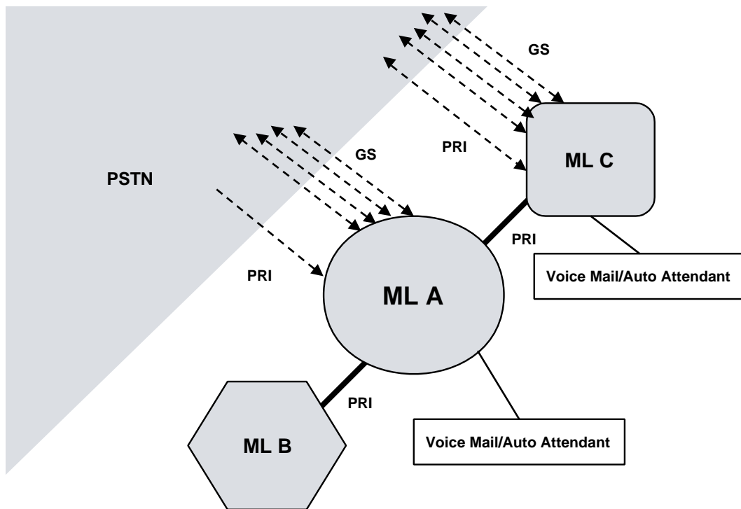
Figure 1-5. Star Configuration: Three Systems
