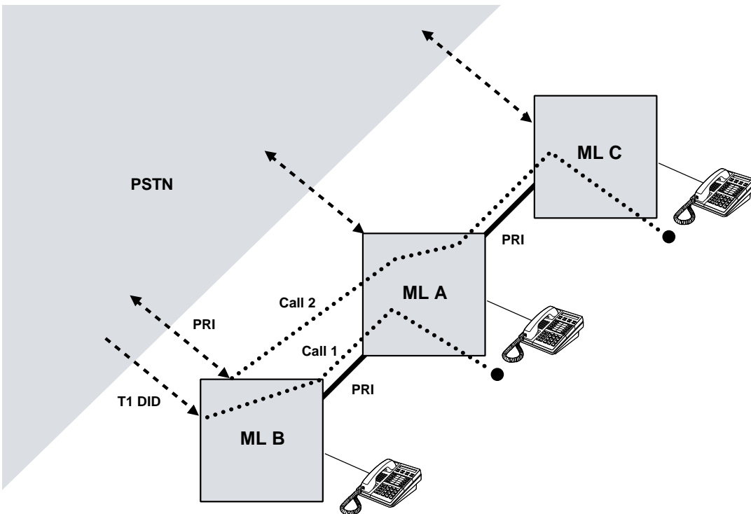
Figure 1-3. Star Configuration: Three Systems
