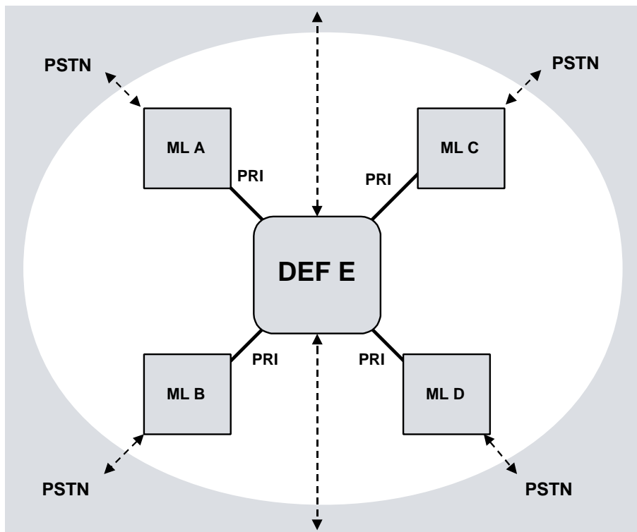
Figure 1-6. Star Configuration: Five Systems
