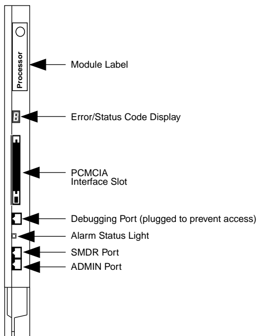
Figure 3-1. Processor Module
