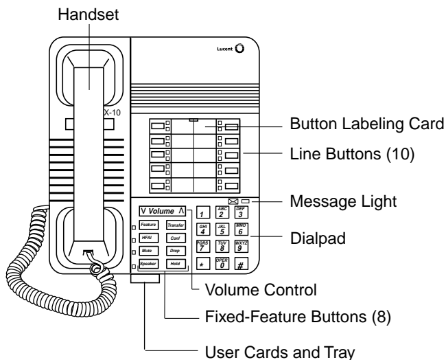
Figure 3-8. MLX-10 Telephone
