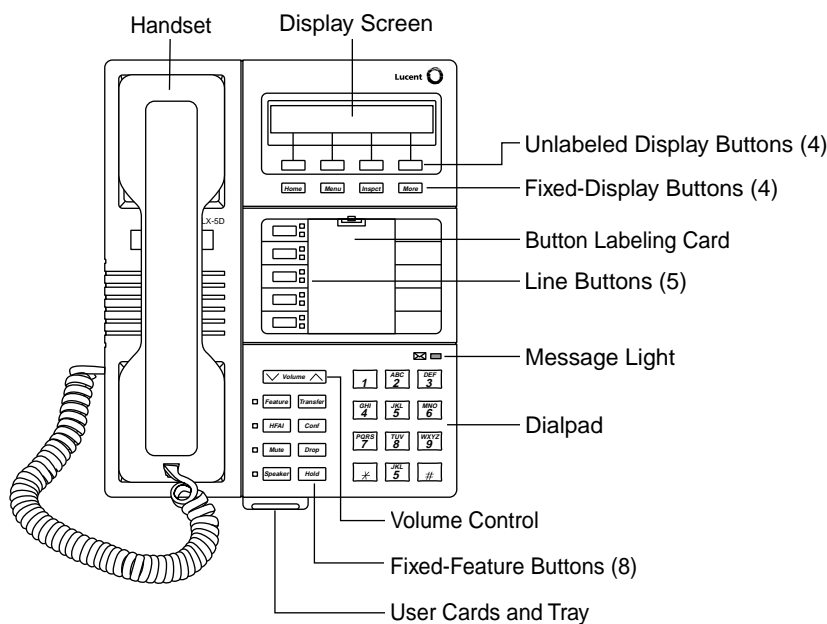
Figure 3-9. MLX-5D Telephone
