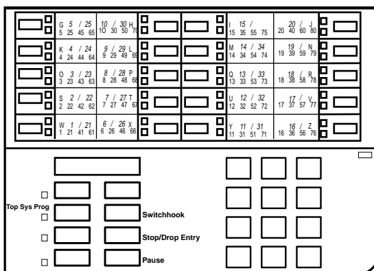
Figure 6-9. Console Overlay
