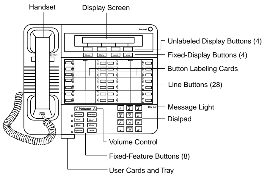
Figure 3-4. MLX-28D Telephone
