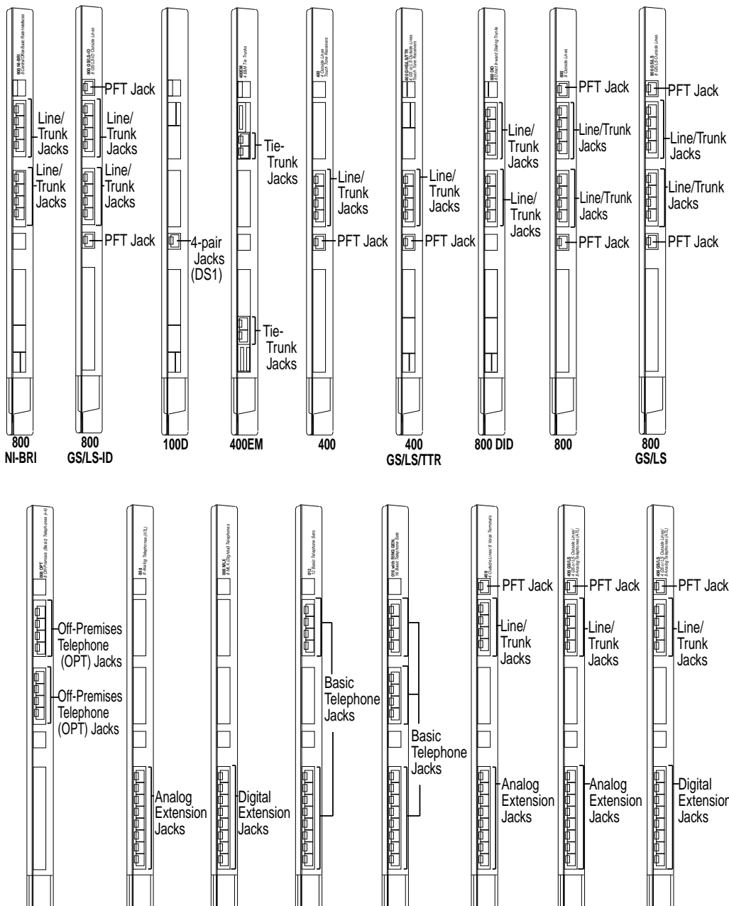
Figure 3-3. Line/Trunk and Extension Modules
