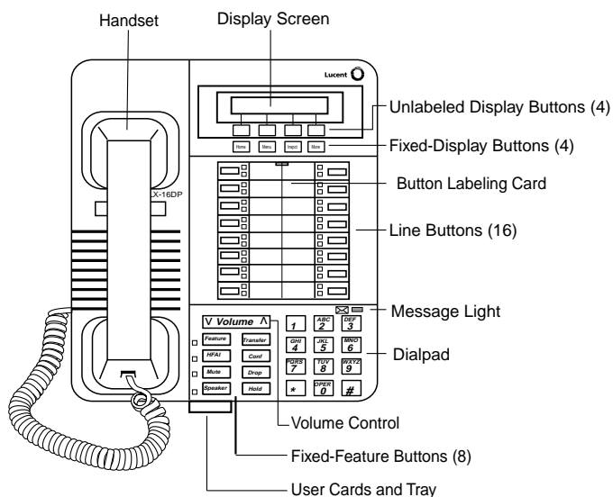
Figure 3-7. MLX-10D Telephone
