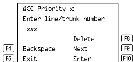
Figure 6-5. Screen Keys
