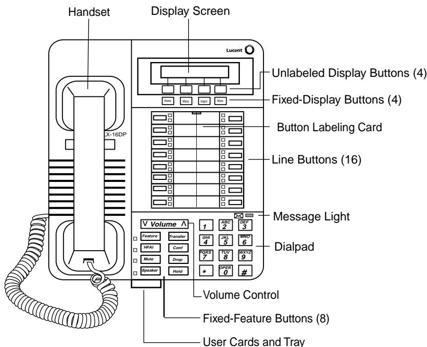
Figure 3-6. MLX-16DP Telephone
