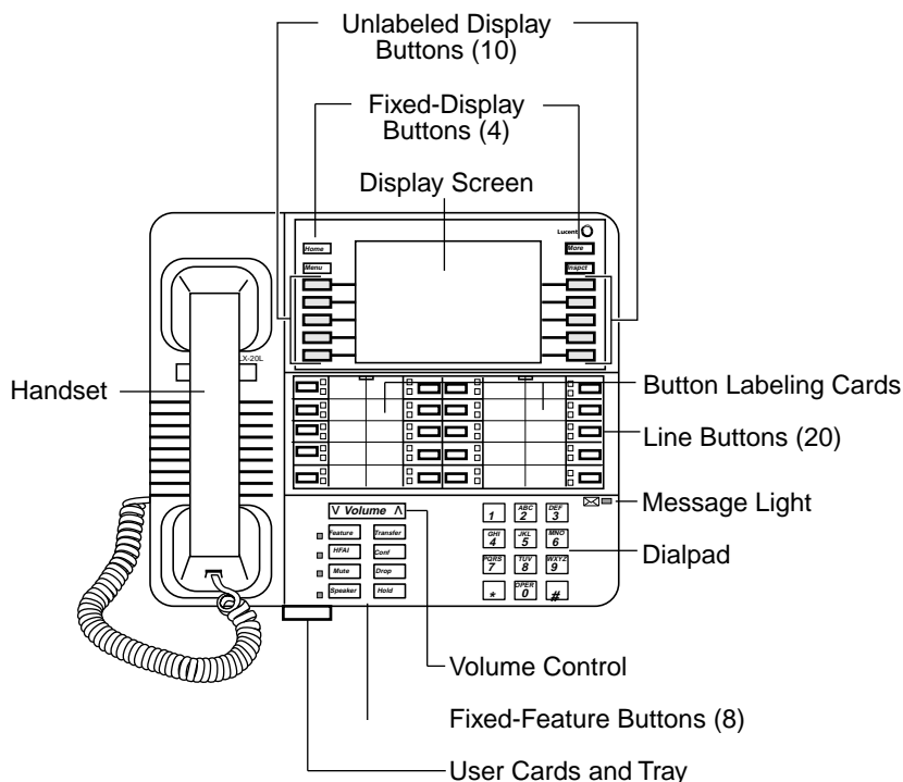
Figure 3-5. MLX-20L Telephone
