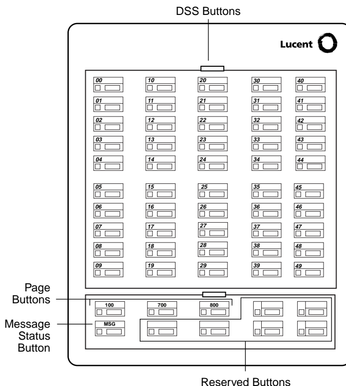
Figure 15. Direct Station Selector (DSS)
