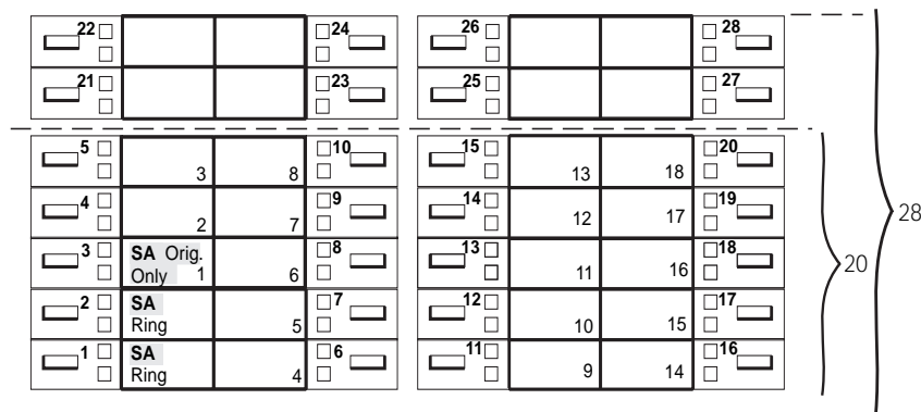
Figure G-1. MLX-20L and MLX-28D Telephone (Hybrid/PBX Mode)
