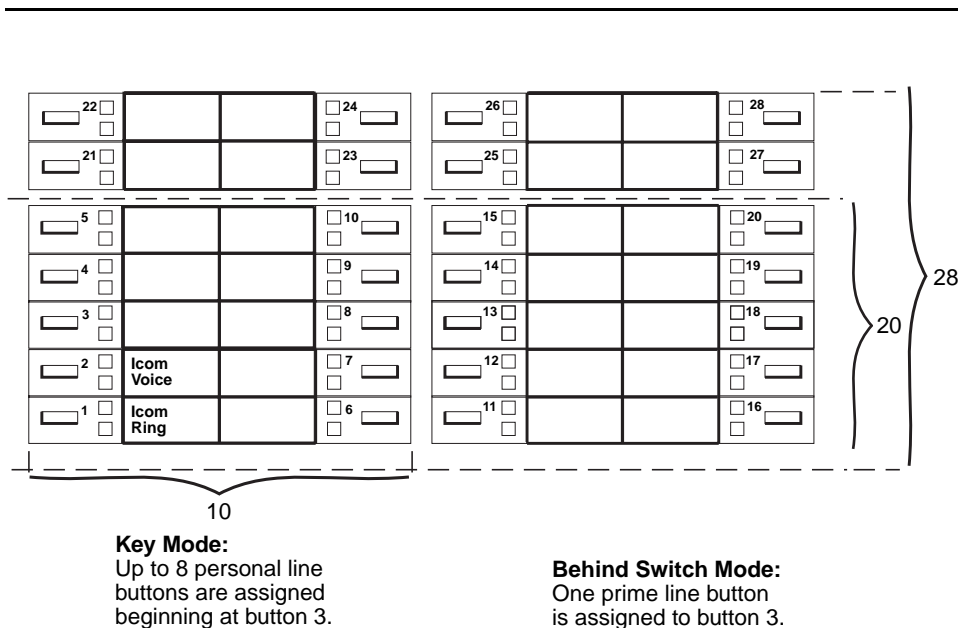
Figure G-5. MLX-20L and MLX-28D Telephone (Key and Behind Switch Modes)
