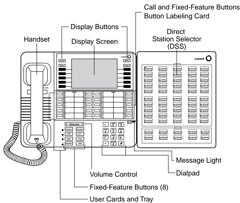
Figure 28. MLX-20L Telephone and DSS
