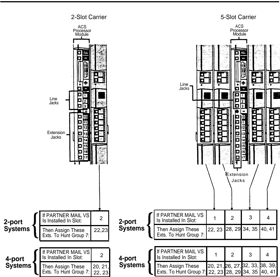
Figure 2-2. Sample Voice Messaging System Extensions for PARTNER Advanced Communications Systems
