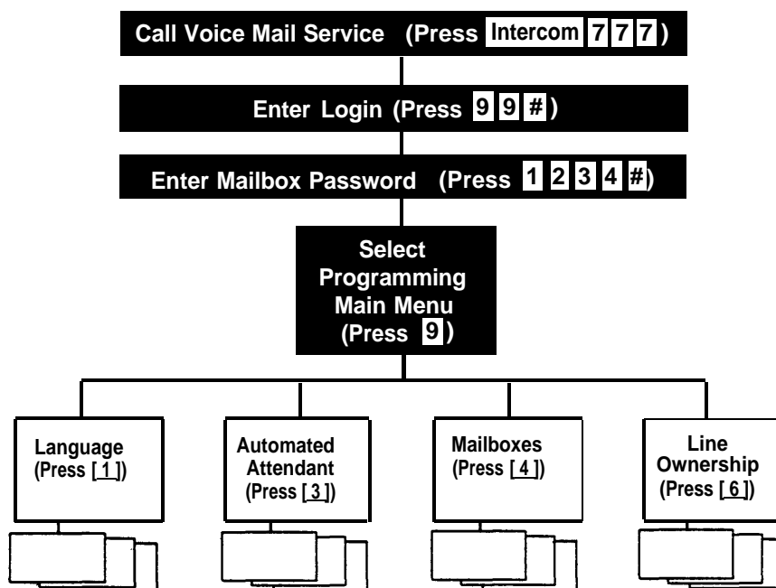
Figure 3-1. Programming Menus
