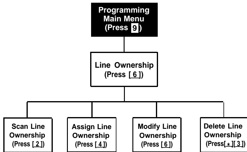
Figure 5-6. Line Ownership
