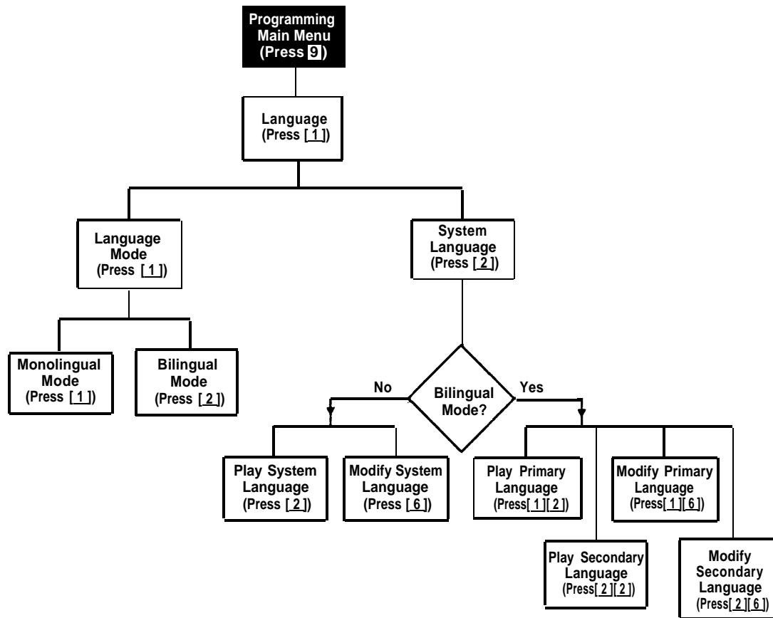
Figure 5-1. Language Menu
