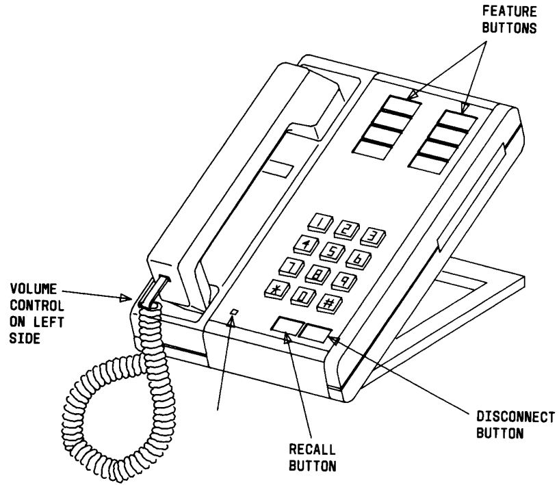
FIGURE 3-3. The 7103A Fixed Feature Voice Terminal
