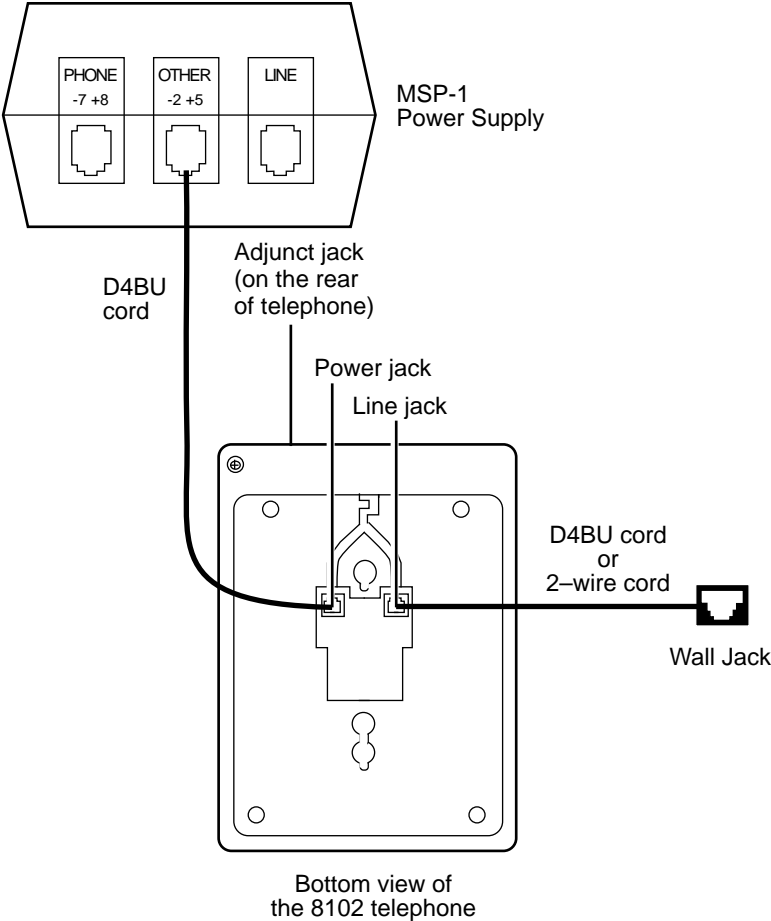
FIGURE 2-6. Local Powering Arrangement for Adjuncts Connected to the 8102 Analog Telephone
