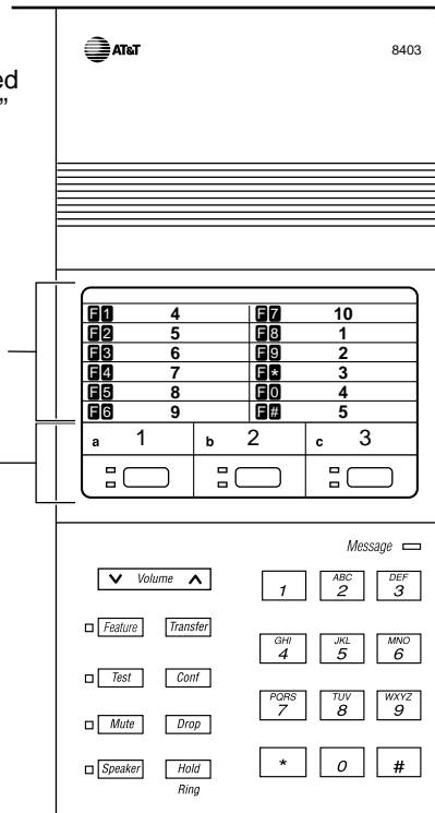
FIGURE 3-45. Button Numbering for Administering the 8403 Voice Terminal Connected to a System 75 or a DEFINITY G1 or G3 Switch
