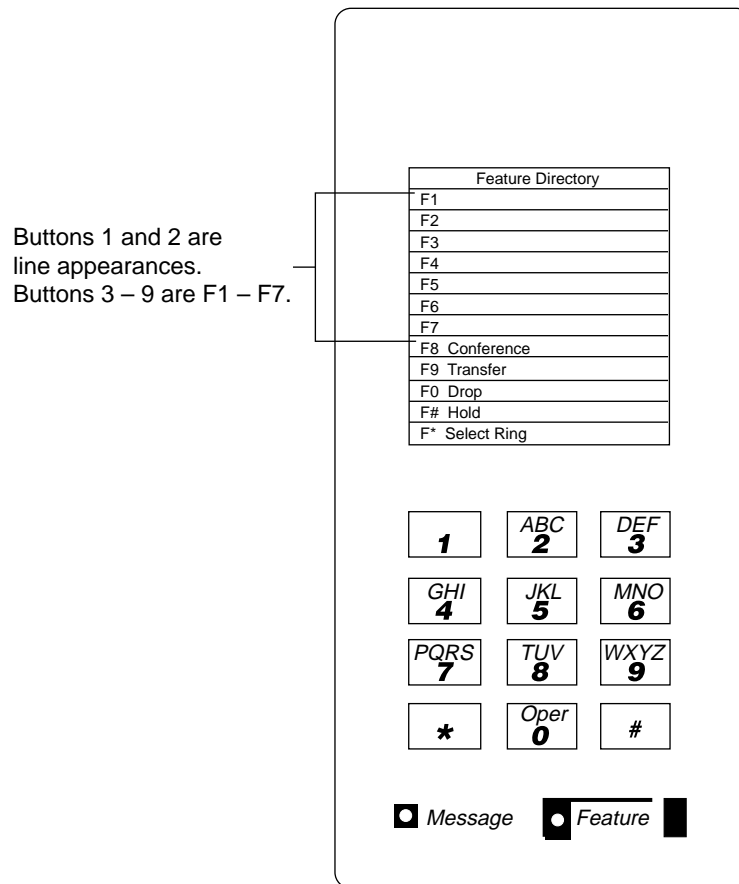
FIGURE 3-10. Button Numbering for Administering the 7401D and 7401 Plus Voice Terminals Connected to a System 75 or a DEFINITY G1 or G3 Switch
