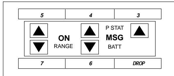
FIGURE 3-25. Button Numbering for a MDC 9000 Connected to System 85 or DEFINITY Generic 2
