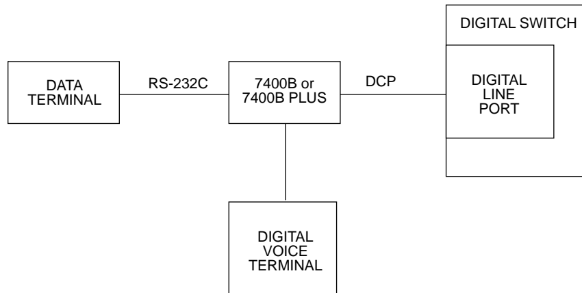
FIGURE 5-2. Block Diagram of the 7400B Interface
