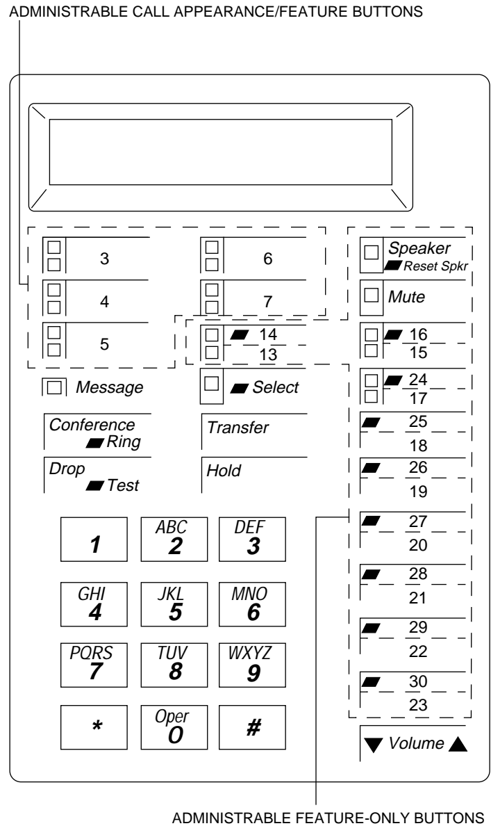
FIGURE 3-24. Button Numbering for Administering the 7406 Plus Voice Terminal Connected to a System 85 or a DEFINITY G2 Switch
