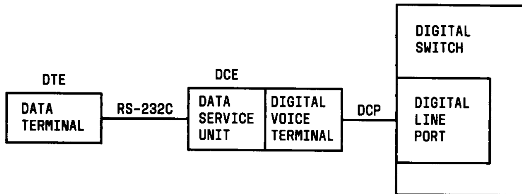
FIGURE 5-2. Block Diagram of 703A Data Service Unit
