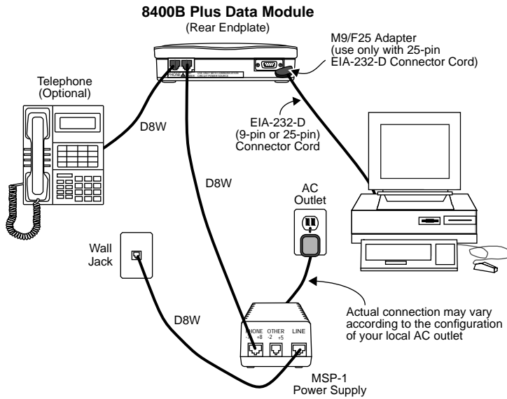
FIGURE 5-3. Typical Installation of the International Configuration, including Telephone and Separate Power Supply
