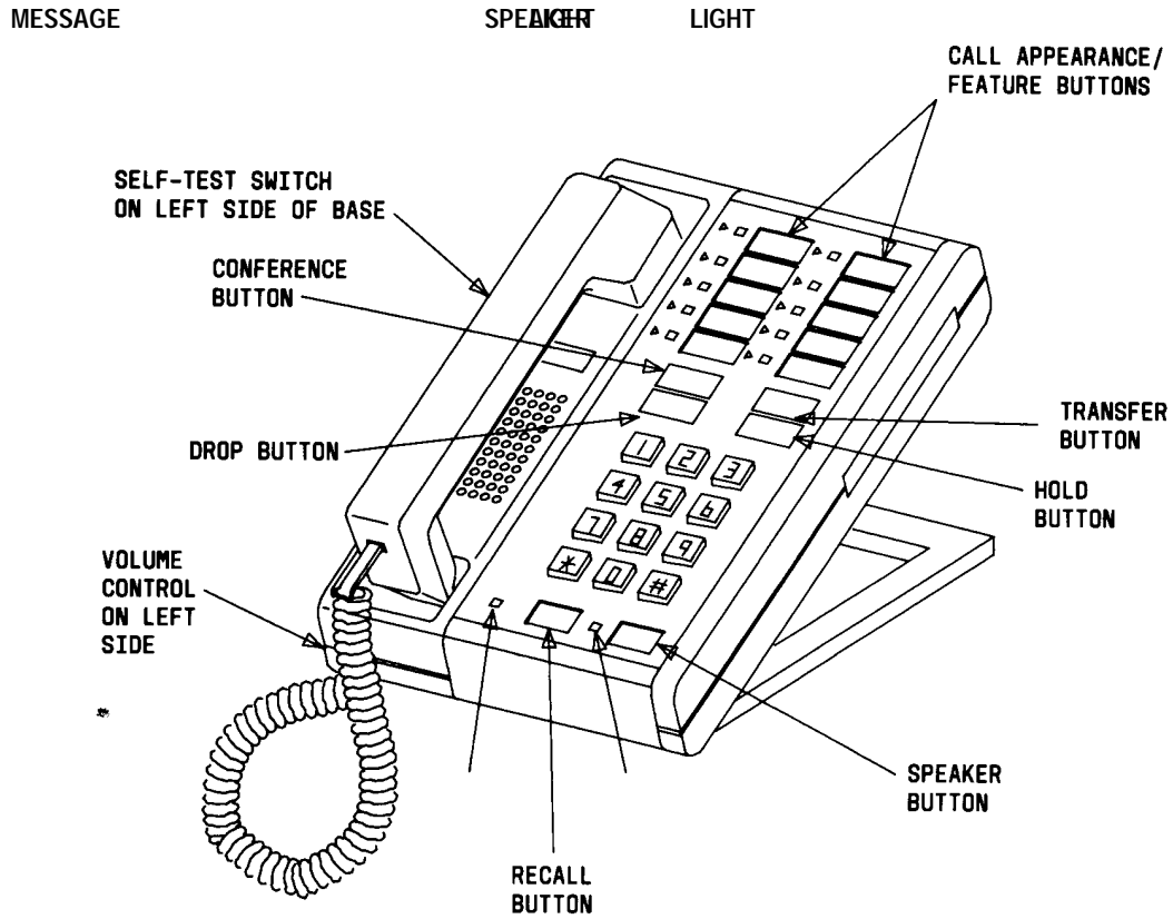
FIGURE 3-7. The 7303S Voice Terminal
