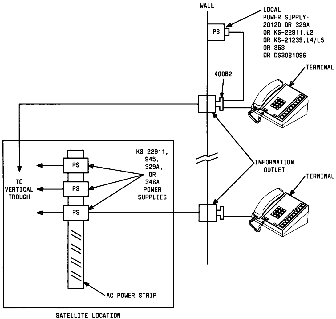
FIGURE 2-4. Local and Satellite Power Sources for Voice Terminals Adjuncts
