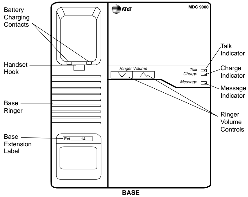
FIGURE 3-23. MDC 9000 Telephone, Top View of Charging Base
