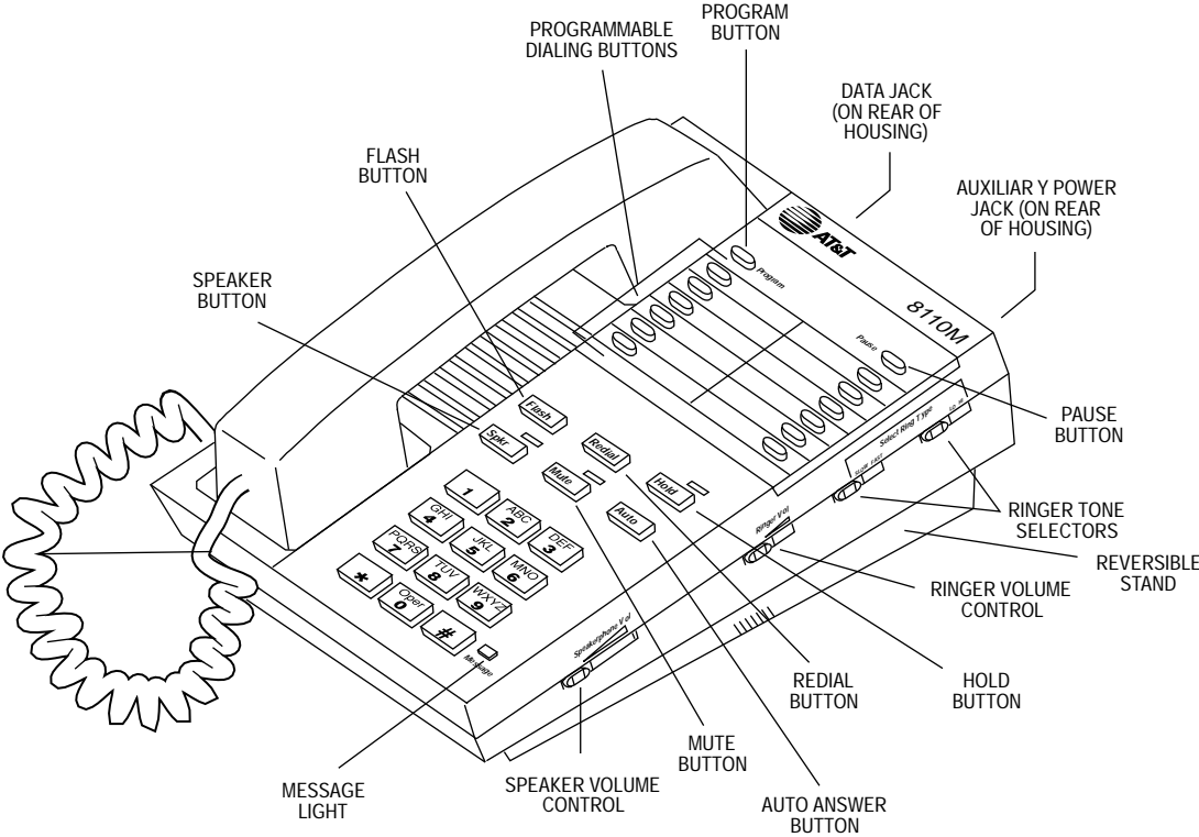
FIGURE 3-14. The 8110 and 8110M Telephones (The 8110M is shown here)
