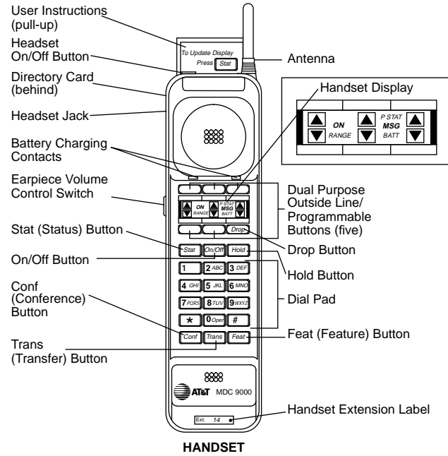
FIGURE 3-22. MDC 9000 Telephone, Top View of Handset, including Enlarged Display Area
