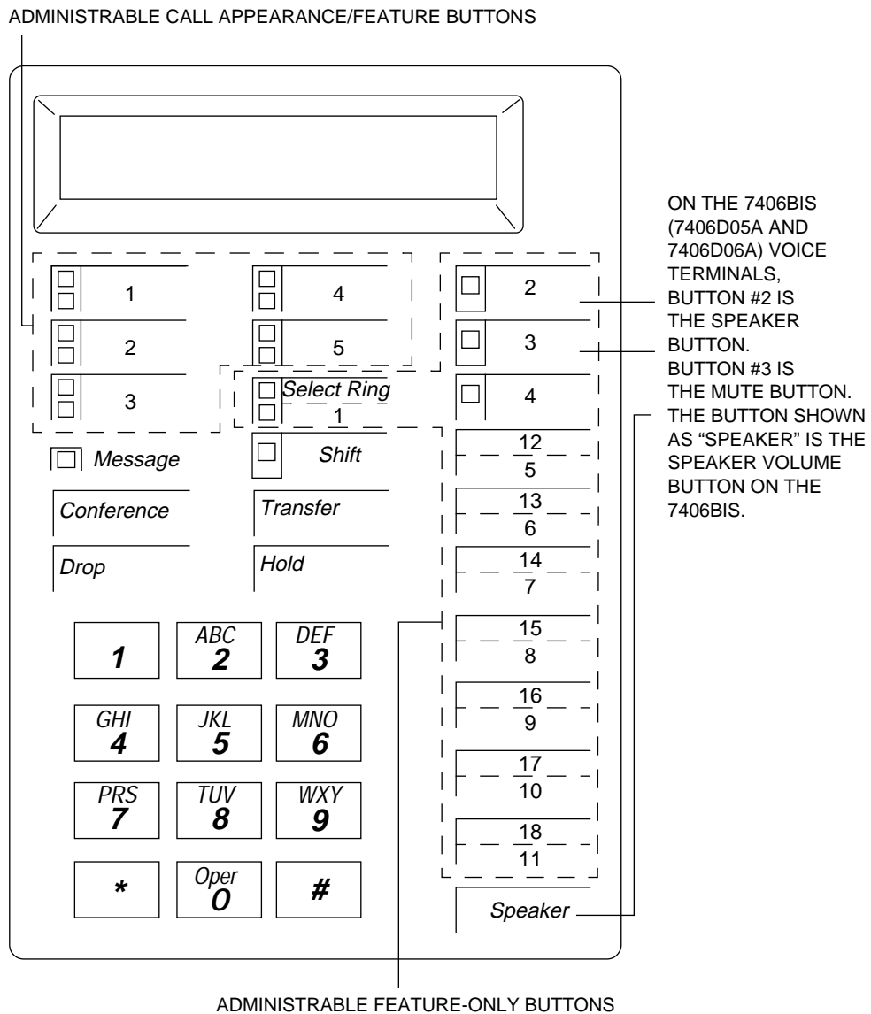
FIGURE 3-21. Button Numbering for Administering the 7406D and 7406BIS Voice Terminals Connected to a System 75 or a DEFINITY G1 or G3 Switch
