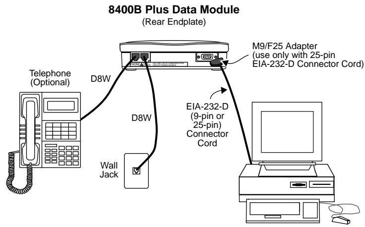
FIGURE 5-4. Typical Installation of the U.S. and International Configuration, including Telephone and Closet Power Supply
