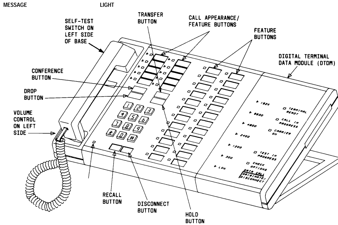
FIGURE 5-6. Digital Terminal Data Module mounted on a 7405D Voice Terminal
