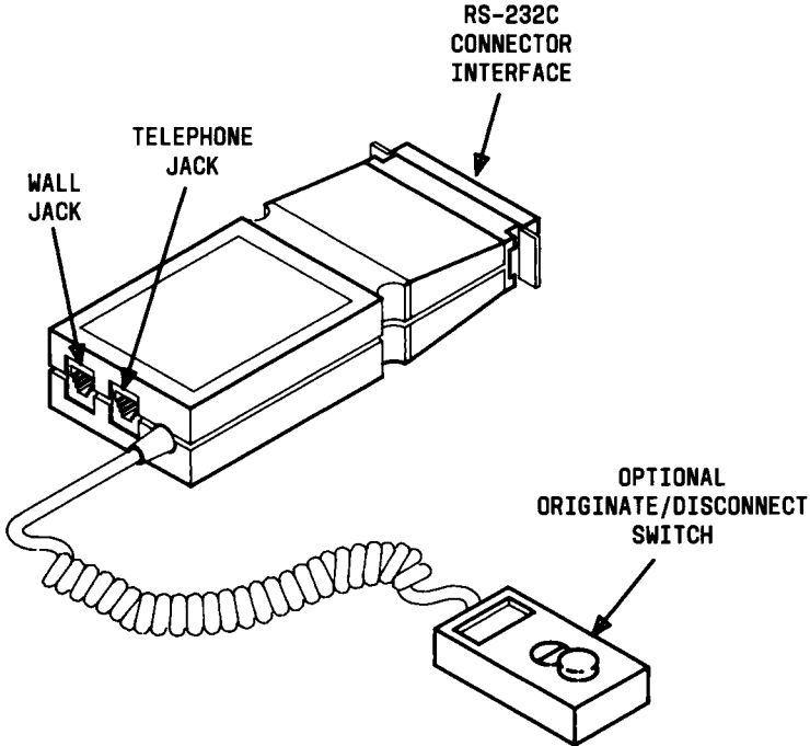
FIGURE 5-3. The Z3A Asynchronous Data Unit
