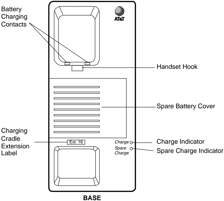
FIGURE 3-27. MDW 9000 Telephone, Top View of Charging Cradle
