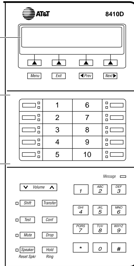
FIGURE 3-48. Button Numbering for Administering the 8410 Voice Terminal Connected to a System 75 or a DEFINITY G1 or G3 Switch
