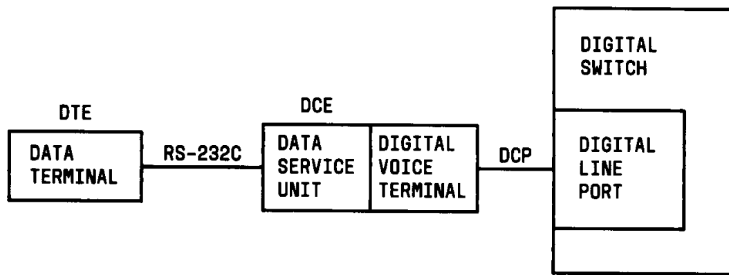
FIGURE 5-2. Block Diagram of Z702AL1 Data Service Unit Interfaces
