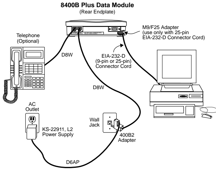
FIGURE 5-2. Typical Installation of the U.S. Configuration, including Telephone and Separate Power Supply
