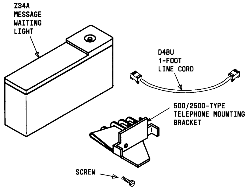
FIGURE 4-4. The Z34A Message Waiting Indicator
