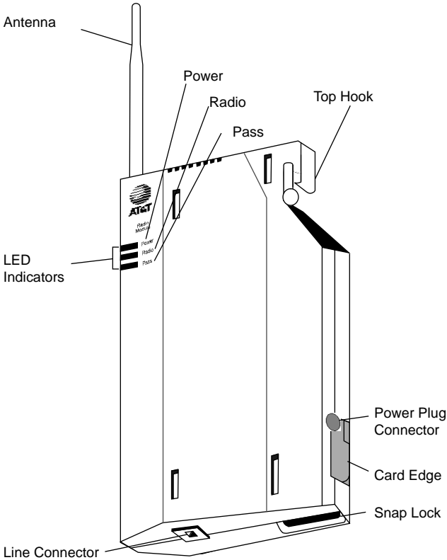
FIGURE 3-28. MDW 9000 Telephone, Radio Module
