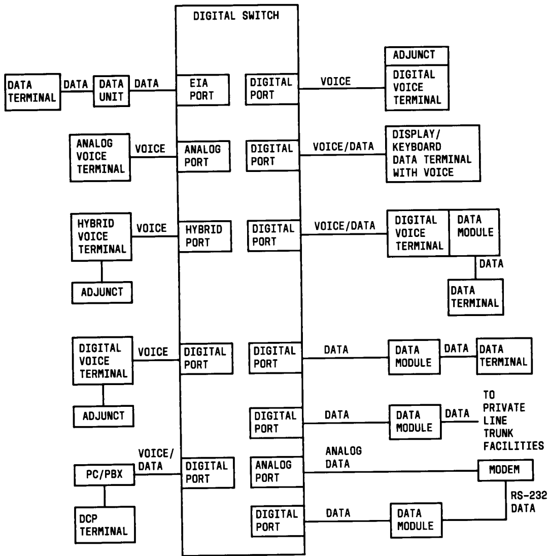
FIGURE 1-1. Interface Between System Switch and Typical Terminals/Adjuncts
