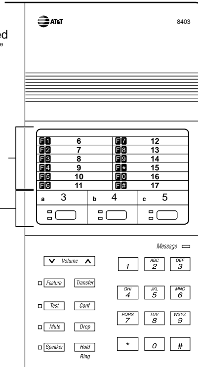
FIGURE 3-46. Button Numbering for Administering the 8403 Voice Terminal Connected to a System 85 or a DEFINITY G2 Switch
