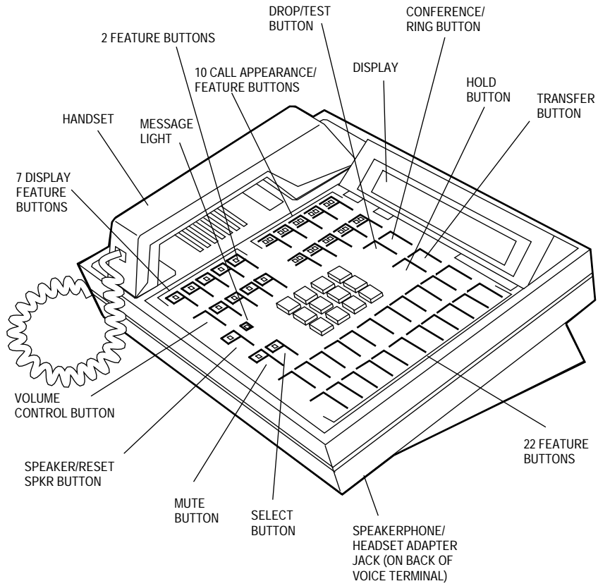
FIGURE 3-27. The 7407 Plus (7407D02D) Voice Terminal
