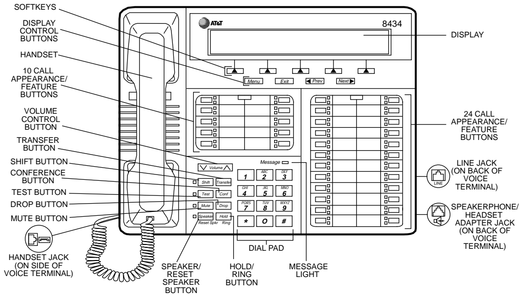
FIGURE 3-50. 8434 Voice Terminal
