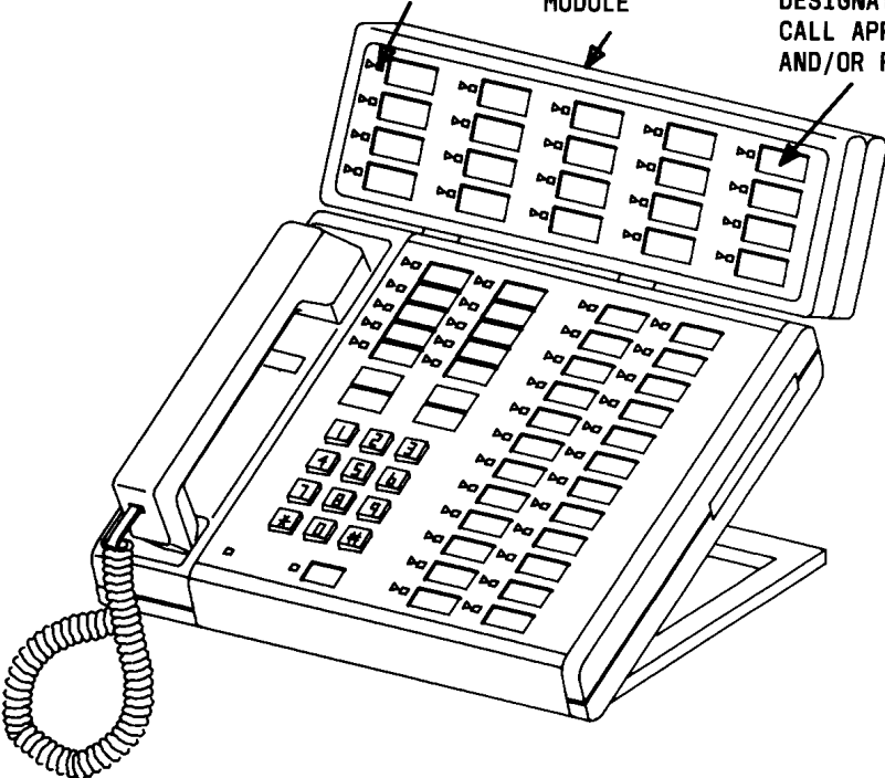
FIGURE 4-1. The C201A Call Coverage Module mounted on a 7434D Voice Terminal
