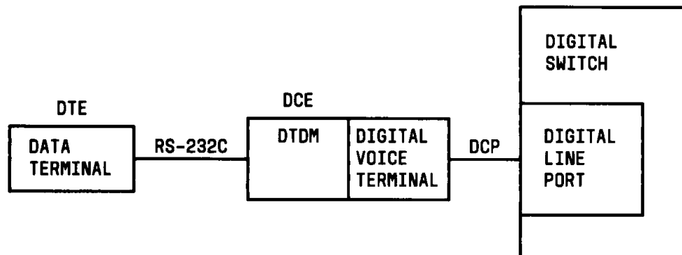
FIGURE 5-2. Block Diagram of DTDM Interfaces
