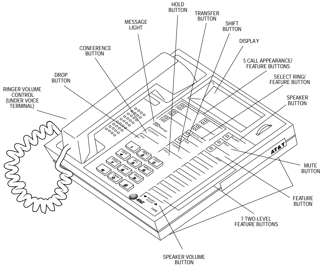
FIGURE 3-19. The 7406BIS (7406D05A) Voice Terminal with Display
