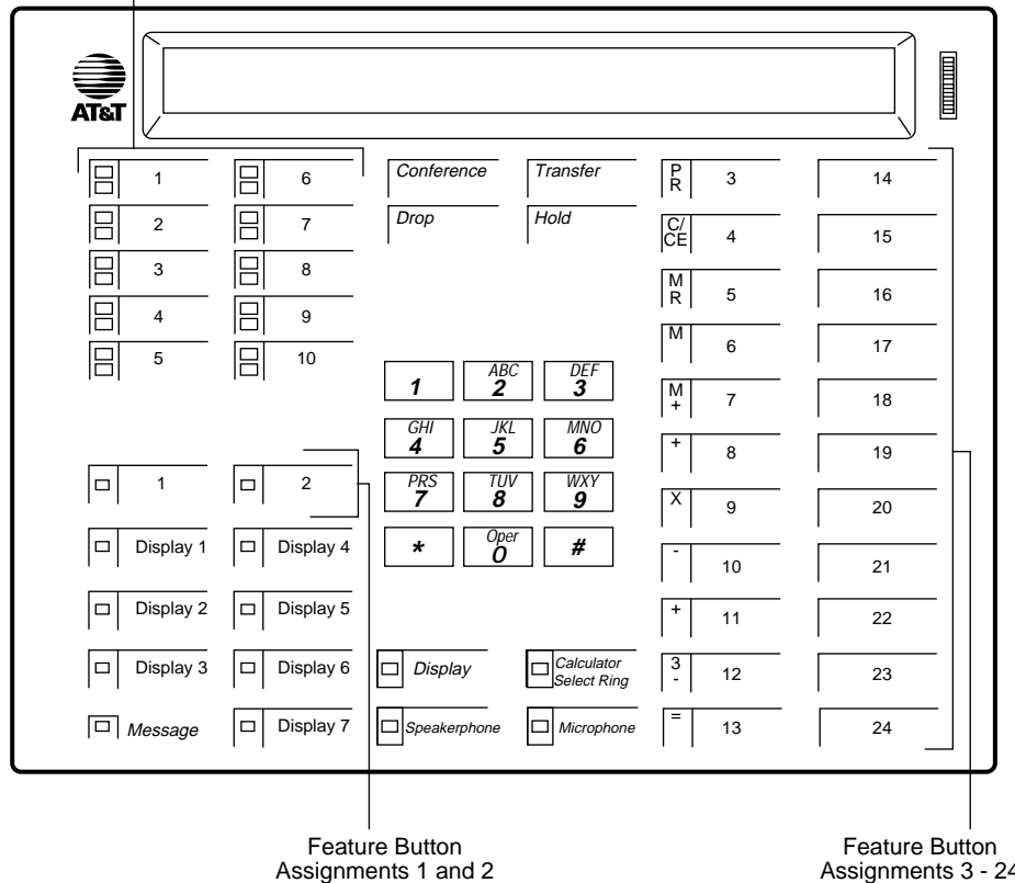
FIGURE 3-28. Button Numbering for Administering the 7407D (7407D01B) Voice Terminal Connected to a System 75 or a DEFINITY G1 or G3 Switch
