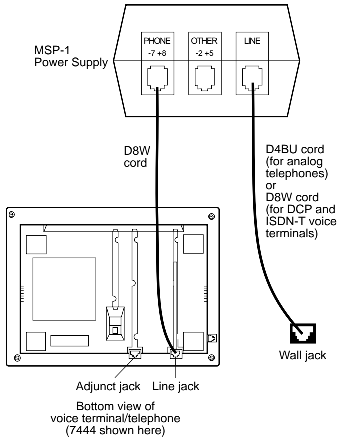
FIGURE 2-5. Local Powering Arrangement for: ISDN-T VTs; the DCP 7444 and 8434 VTs (for their VF Displays); and Adjuncts Connected to All Telephones Except the 8102
