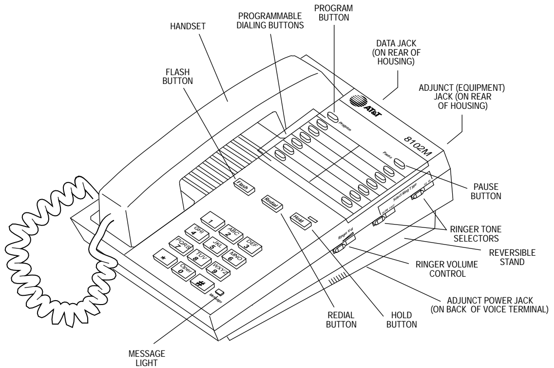
FIGURE 3-13. The 8102 and 8102M Telephone (The 8102M is shown here)
