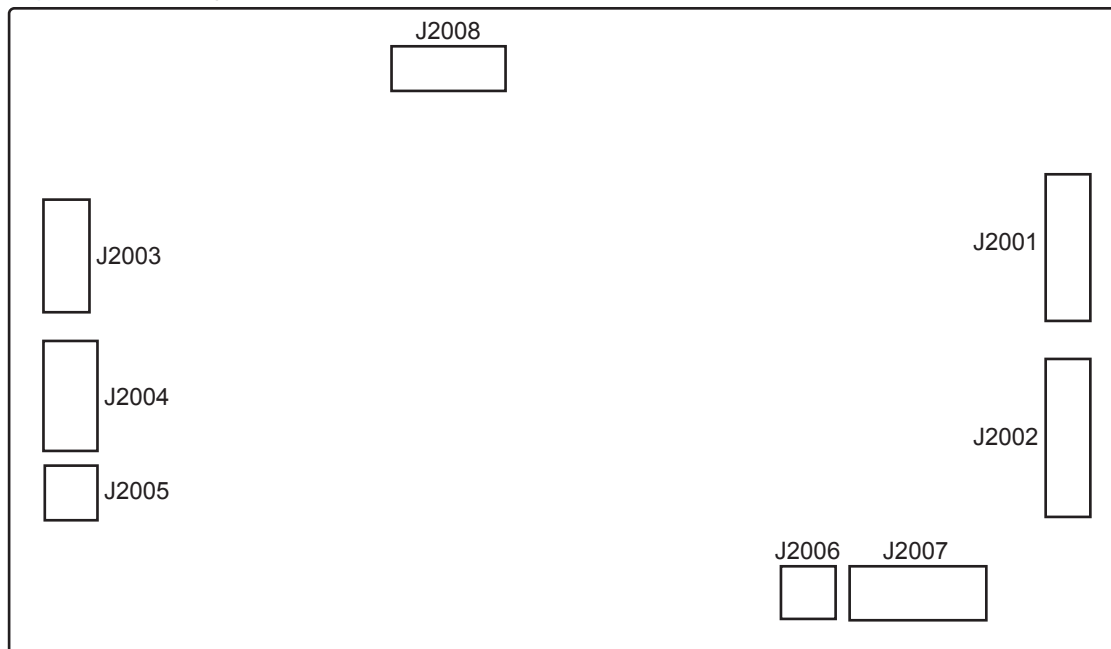
Figure 2-17 Paper Deck Controller PCA
