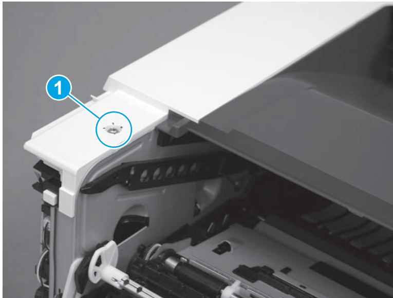
Figure 1-1306 Install one screw
