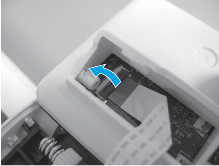
Figure 1-2165 Release the FFC and remove the control panel
