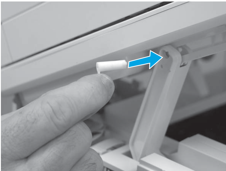
Figure 1-573 Install the slider pin
