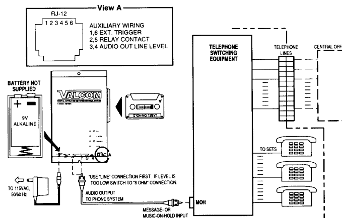
Typical Telephone System Connection Diagram
