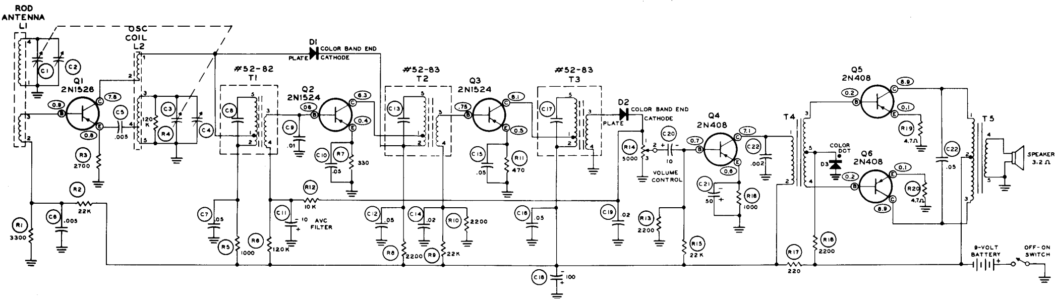
SCHEMATIC OF THE HEATHKIT PORTABLE TRANSISTOR RADIO MODEL GR-151A
