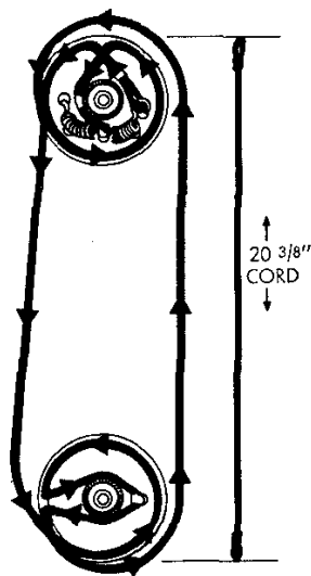
SYNTHESIZER TUNE DRIVE CORD DRIVE PULLEYS SHOWN AT MAXIMUM COUNTERCLOCKWISE ROTATION
