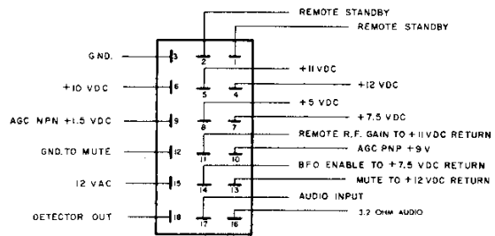
J-14 ACCESSORY SOCKET
