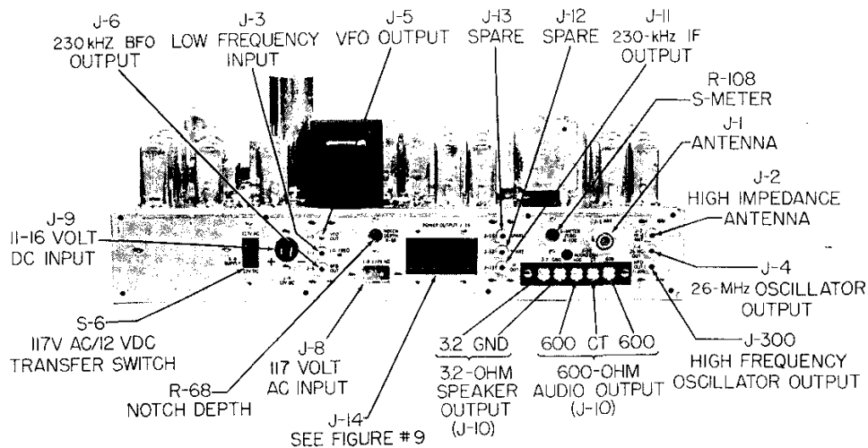
HRO-500 RECEIVER, REAR PANEL
