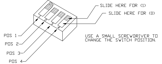
Switch (SW1) Settings
