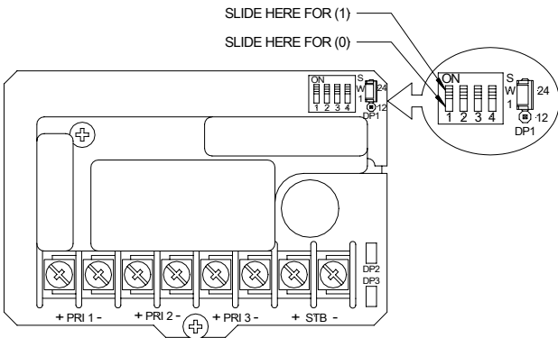
Figure 1. PC Board Layout Showing Location of Jumper Plug (DP1) and Switch (SW1)
