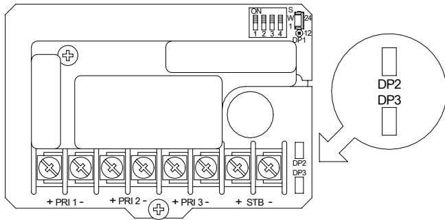
Figure 4: PCB Layout Showing Location Of Jumper Plugs DP2 & DP3
