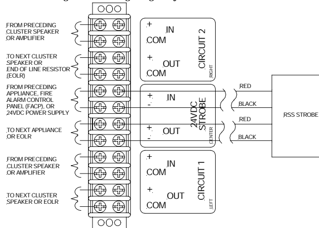
Figure 3: Wiring Diagram for Two Audio Circuits
