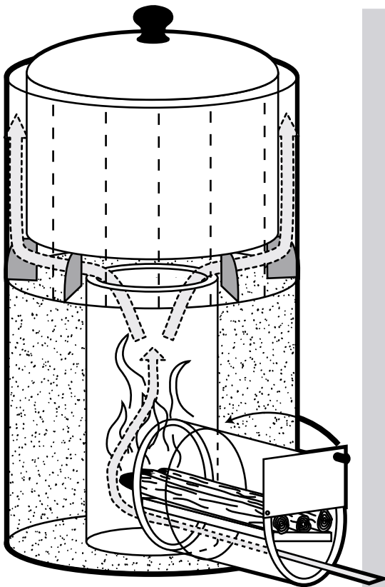
Winiarski Rocket Stove (page 30)
