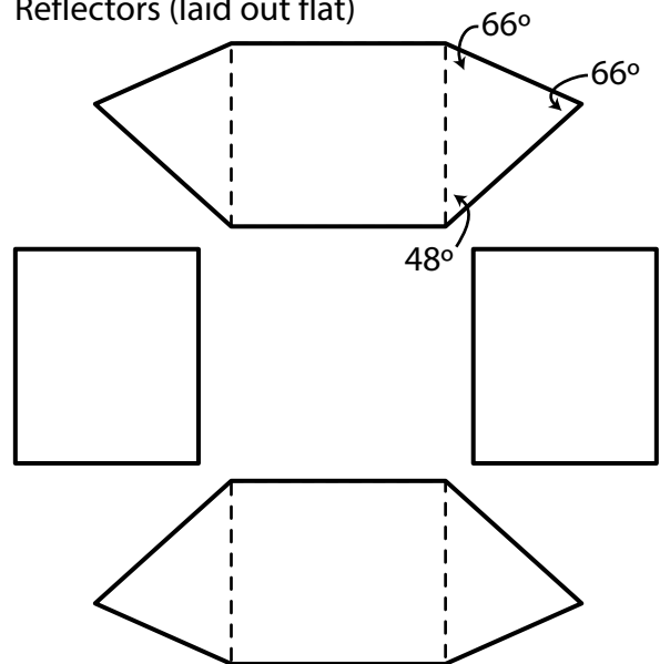
Reflectors (laid out flat)
