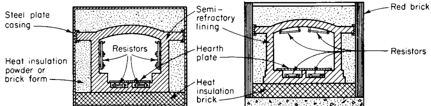
Fig. 7.5.1 Heating chamber with sidewall and hearth resistors.
