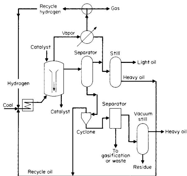
Fig. 7.1.5 H-coal schematic.
