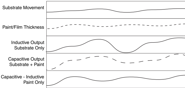
Figure 8.7.23: Combining inductive and capacitive technologies in one application to measure film or paint thickness on a metal substrate
