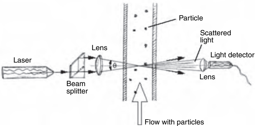
Figure 10.1.7: LDA configuration.
