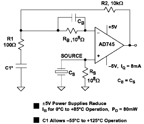
Figure 4.4.31: Gain of 100 piezoelectric sensor amplifier.
