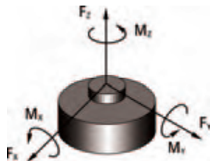
Figure 11.3.3: Load cell axis definitions.
