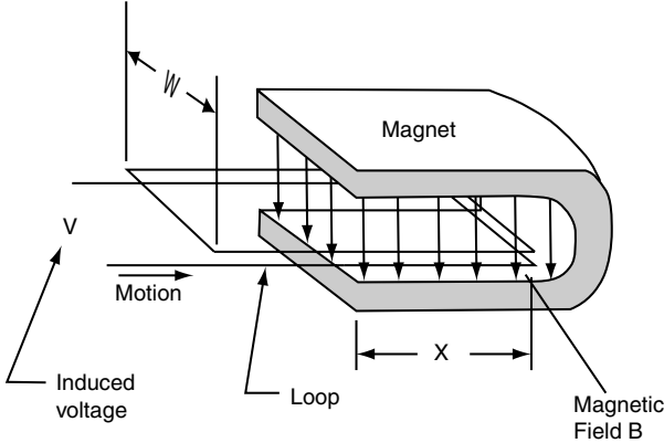
Figure 9.3.1: Magnetic sensor.
