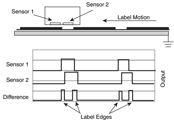
Figure 8.7.16: Differential capacitive measurement senses the gap between labels on a web.
