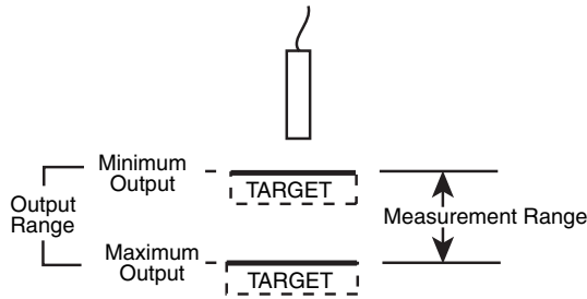
Figure 8.5.1: How the “Output” and “Range” of a sensor relate to target position.
