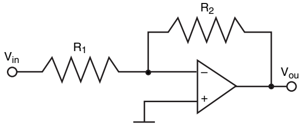
Figure 1.1.8: Inverting amplifier.
