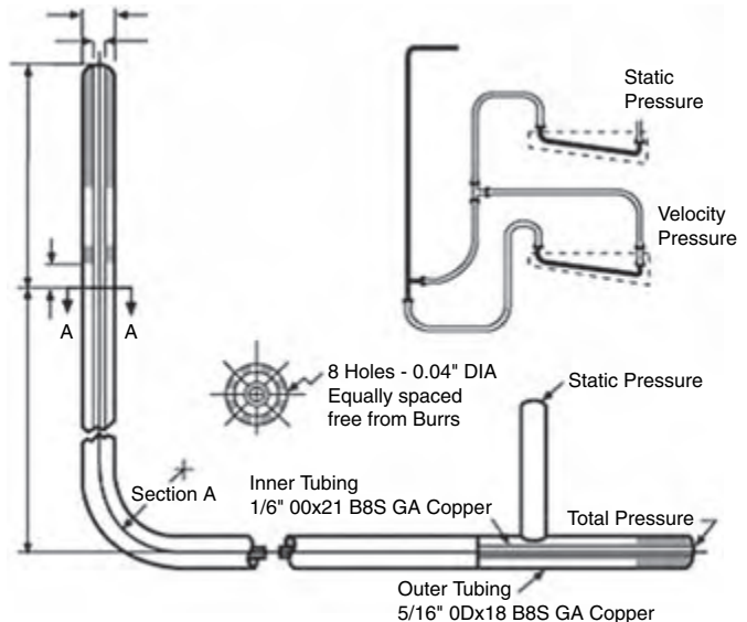
Figure 10.1.1: The Pitot tube.
