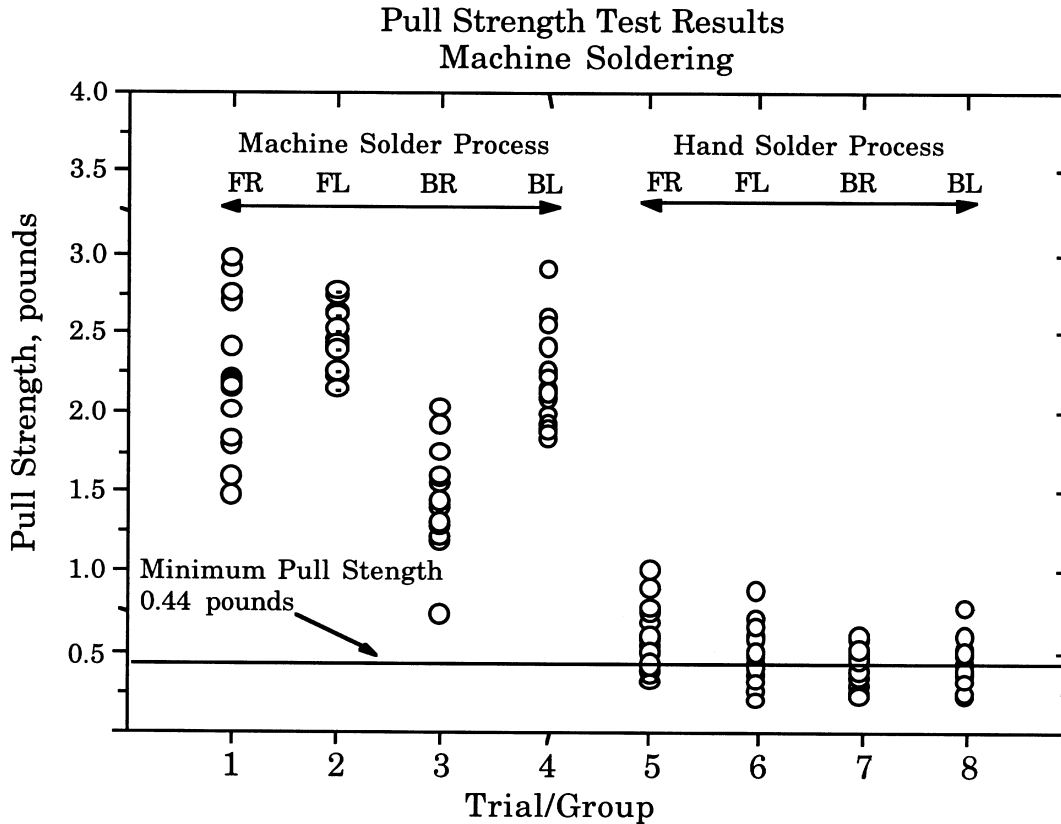
Figure 32, Pull Strength
