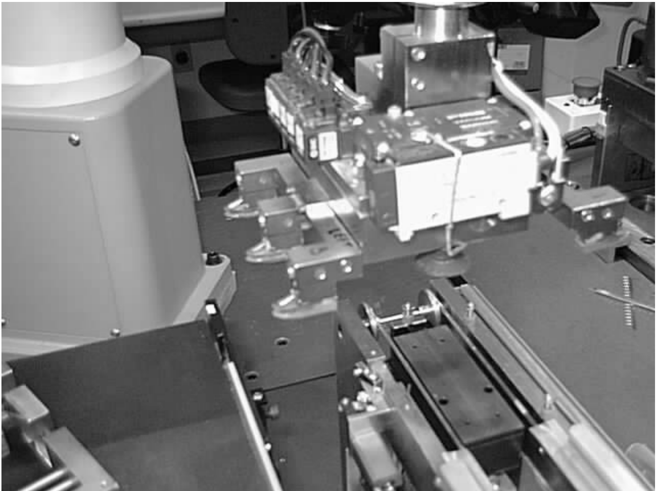
Figure 25, End Effector
