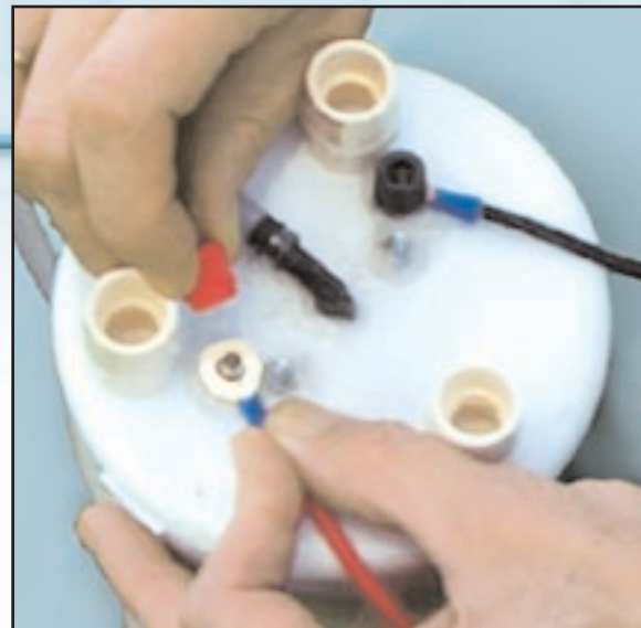
Attaching connections. The electrolyzer is upside down.
