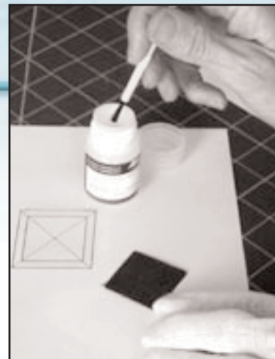
Coat the loaded carbon cloth with Nafion solution
