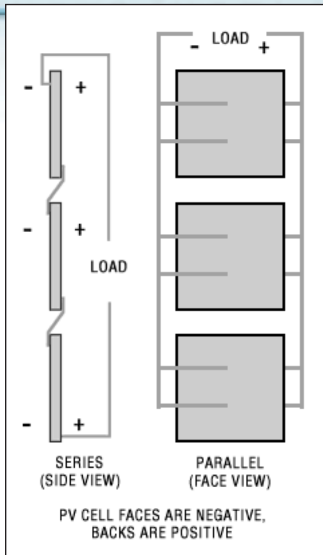
PV cell connections
