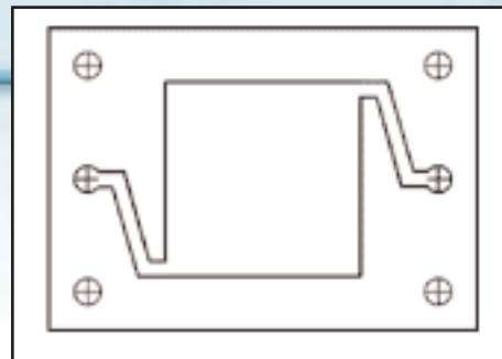
Surround gasket with gas distribution area
