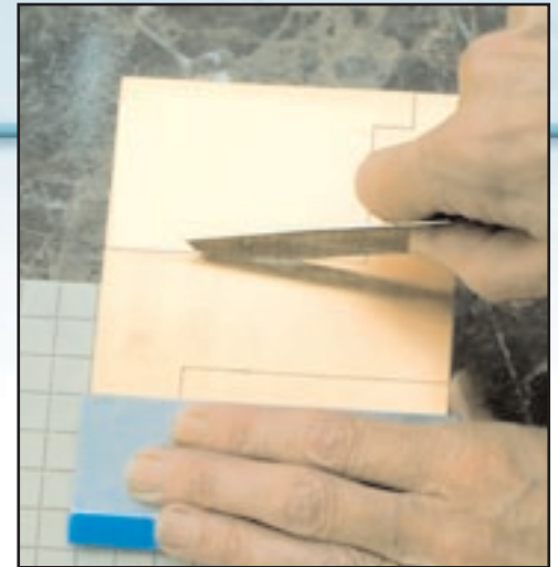
Cutting the endplates from the circuit board
