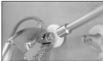
Hold the element connector with locking pliers when removing and installing the connector.
