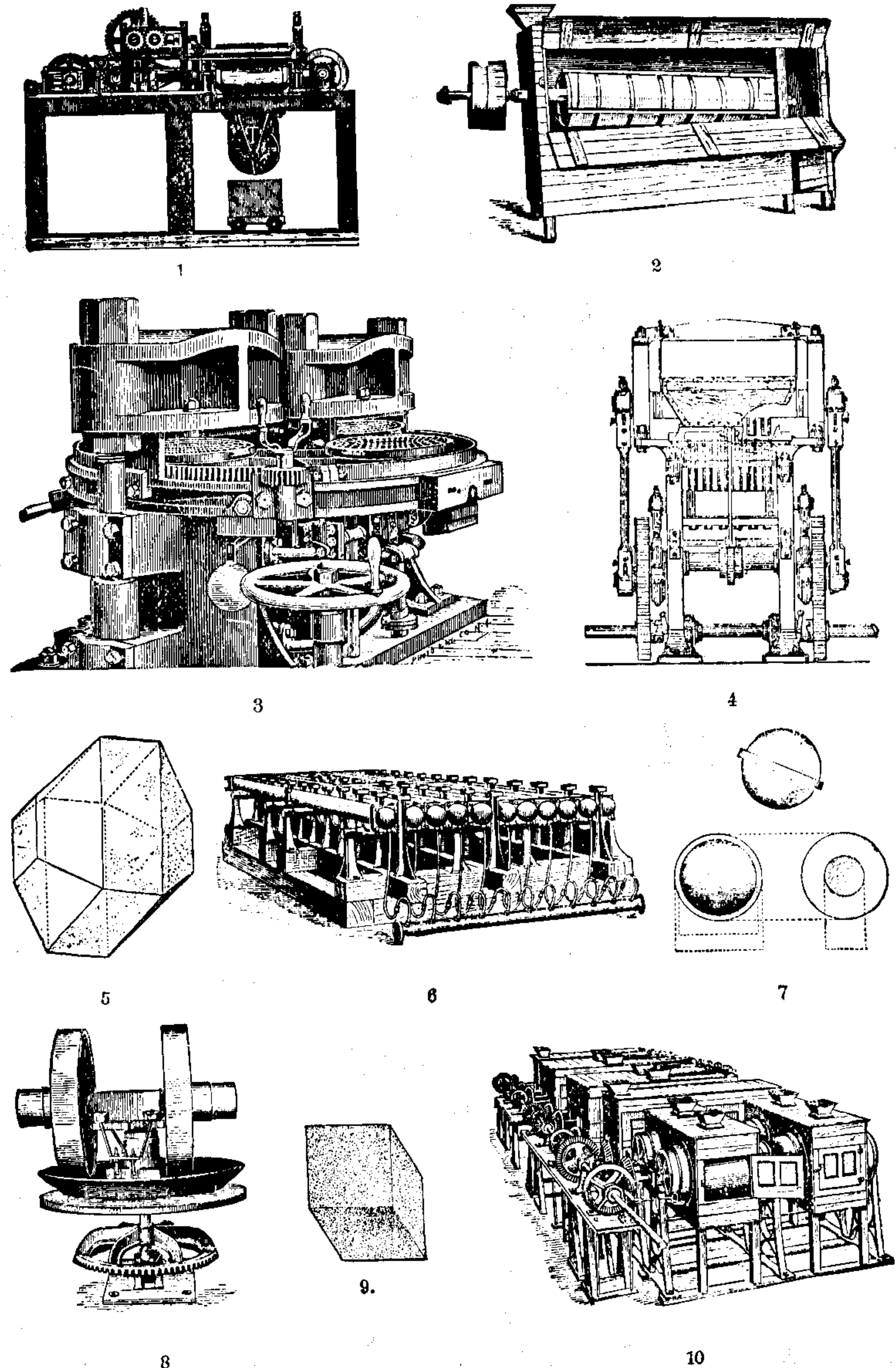
GUNPOWDER.—1, Pebble Powder Machine. 2, Sifting-reel. 3, Pellet Powder Machine. 4, Prismatic Powder Machine. 5, Schaghticoke Powder. 6, Drying-stove. 7, Compensating Powder. 8, Saltpeter Apparatus. 9, Cubical Powder. 10, Dusting-reels.
