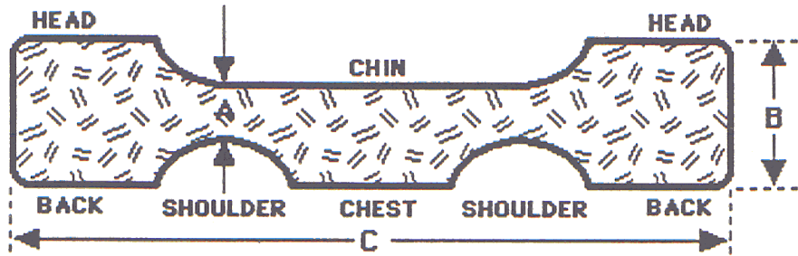
NECK PROTECTOR: Protects the neck, upper chest, back of the head and upper back. A=Neck length. B=Depends upon desired coverage of back of head, upper back and chest. C=Circumference of neck + 2".
