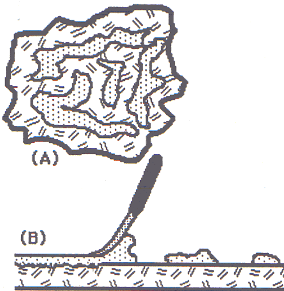
DISPENSING SILICONE SEALANT: (A) Beads of sealant on the felt. (B) Spreading the sealant with the putty knife. Sealant is mashed into the felt fibers. Allow 24-48 hr for curing.
