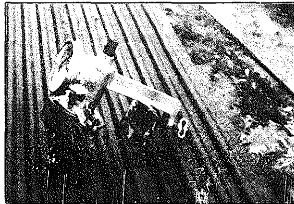
Quaker City mill showing steel plate brazed onto cast-iron grinder base to extend stability and support. Shown resting on trailer plate coil.
