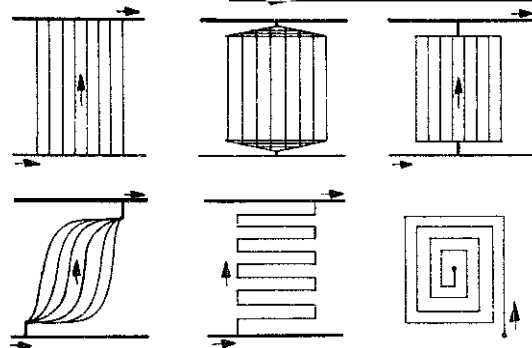
Various tube configurations for solar absorber surfaces.
