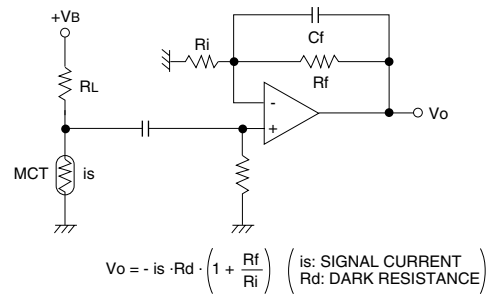
Figure 8-7 Basic operation circuit
